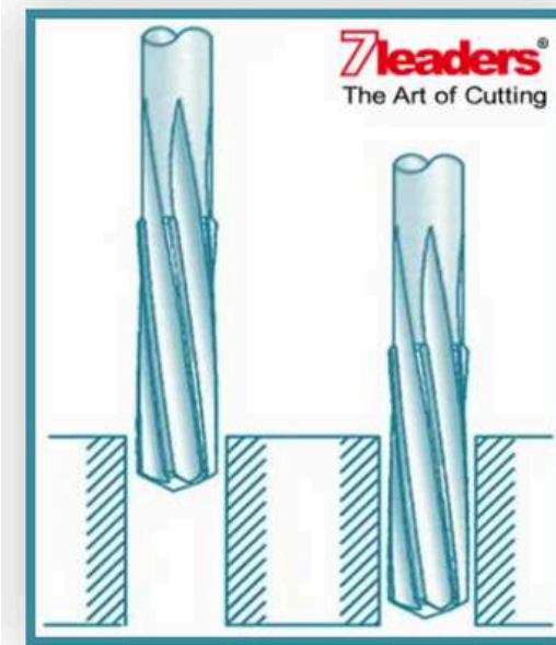
Reamers
